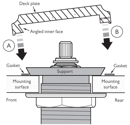
Fitting the deck plate
