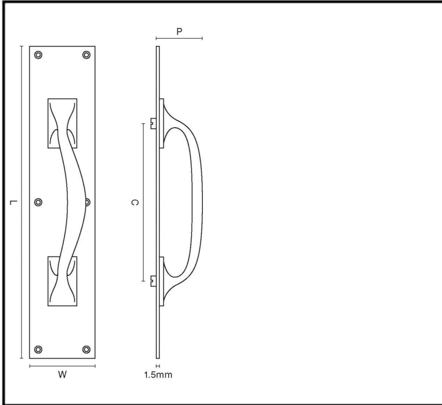
Pull Handle On Plate 1651
