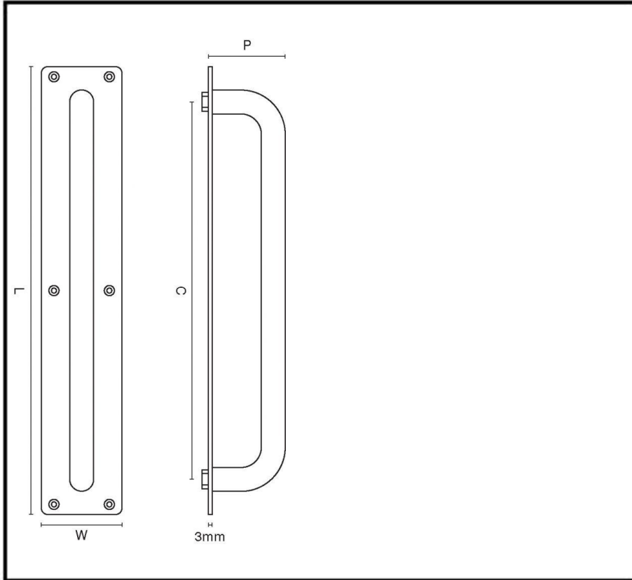
Pull Handle On Plate 1691
