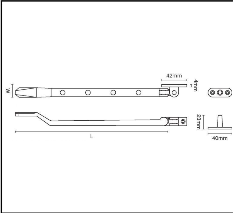
Art Deco Casement Stay 7017
