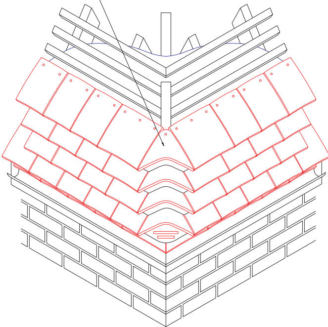
Bonnet hip tile
