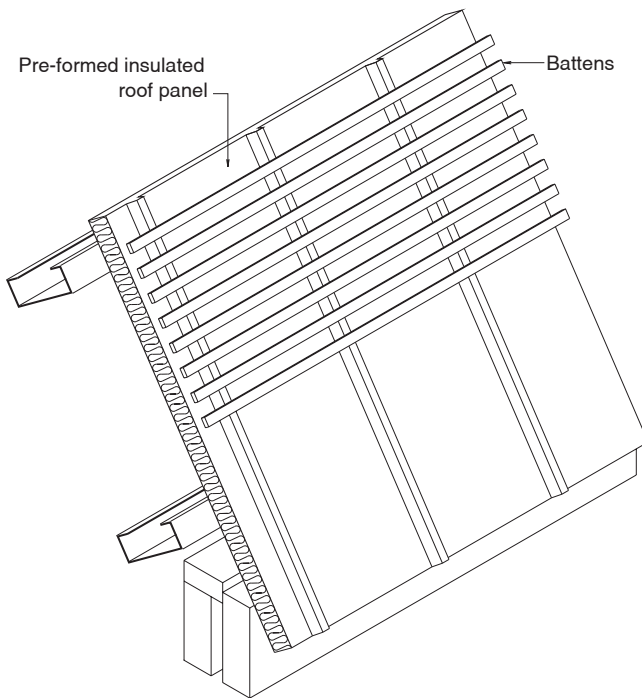
Section through inclined roof structure
