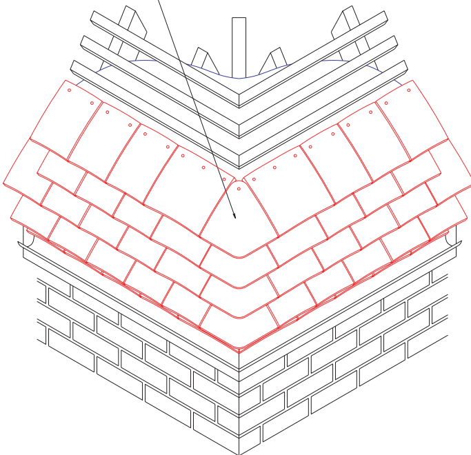
Arris hip tile
